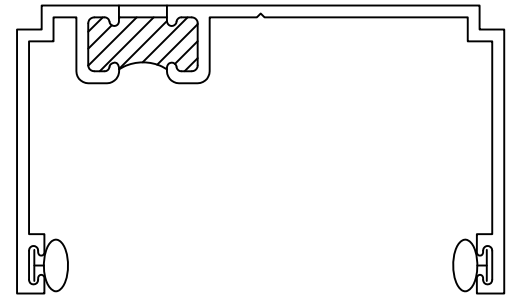
ONE PIECE RECEPTOR SYSTEM FOR 2" WINDOW (PART #30080)
